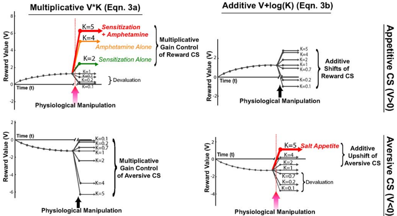
Figure 1. Simulations of dynamic shifts in incentive saliency. All are induced by changes in physiological state after learning a CS-UCS association in an initial state (Eqn 3). The left column is for multiplicative mechanisms (Eqn 3a), while the right column is for additive mechanisms (Eqn 3b). The top row is for shifts after learning a Pavlovian association with a reward UCS (e.g., sucrose taste), and the bottom row is for shifts after learning with an aversive UCS (e.g., intense salt taste). Initial learning is assumed to proceed by a Rescorla-Wagner type of rule initially [20] ( t = 0, 1, \dots, 10 ) as described by the equation V(t) = A(1 - \exp(-t/\tau)) , with asymptote A = 1.3 for appetitive reward and A = -1.3 for aversive reward, and the time constant \tau = 3 . At time step t = 11 , a new motivation manipulation is introduced, such as by a shift in a physiological state relevant to the reward. The change in incentive salience occurs as indicated by the arrows, either multiplicatively ( V \cdot \kappa ) or additively ( V + \log \kappa ), where \kappa (for illustrative purpose) takes the values 5, 4, 2, 1, 0.7, 0.2, 0.1. See Eqn (3a,3b) of the manuscript. Colored lines in the upper-left panel describes Experiment 2 (drug sensitization and acute amphetamine administration), while the lower-right panel depicts Experiment 1 (salt appetite). Note that additive modulation can reverse reward valence, while multiplicative modulation maintains the original reward valence and changes only magnitude.
